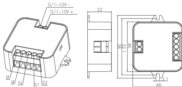
Fixture mounting HBTD8200V/F
