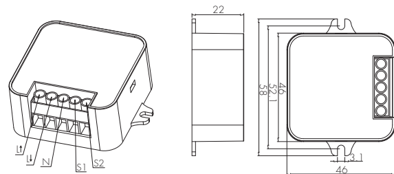
Fixture mounting HBTD8200S/F
