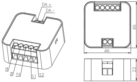
Socket mounting HBTD8200D
